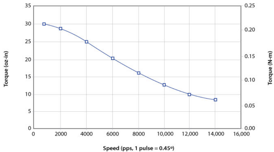
4209S-01S 24VDC, 0.67 Amps/Phase, Bipolar Series, 1/2 Stepping
